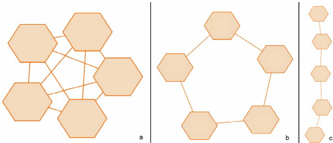
Figure 1: Illustrations of the average minimum graph distance (AMGD). The figure shows some simple graphs, where lines between nodes indicate adjacency. The graph in panel a has AMGD = 1 , the graph in panel b has AMGD = 1.5 and the graph in panel c has AMGD = 2 . Graphs rendered with aiSee v. 2.2.
