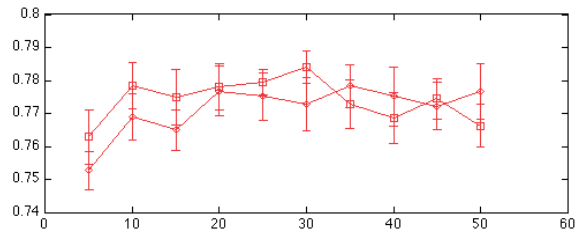
Figure 3: F measures for the blended (i.e., equally weighting areas and domains) and normalized matrix for varying k (x-axis) for SVD (squares) and NMF (diamonds). Remarkably, with normalization, the performance does not drop off much at all with more dimensions, suggesting that previous results about the true number of subcomponents of brain activity may simply be a result of oversampling particular kinds of experiments. Normalization also appears to eradicate any difference in performance between the two methods. (Graph scaled to match previous figure.)
