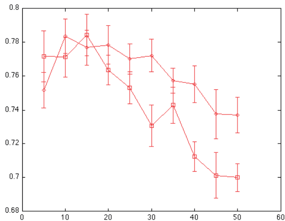
Figure 2: F measures for the blended (i.e., equally weighting areas and domains) unnormalized matrix for varying k (x-axis) for SVD (squares) and NMF (diamonds). Overall performance is better once the two data sources are weighted to contribute equally, and predictive performance with more dimensions does not suffer as much. NMF benefits most from the weighting, now outperforming SVD with more dimensions.
